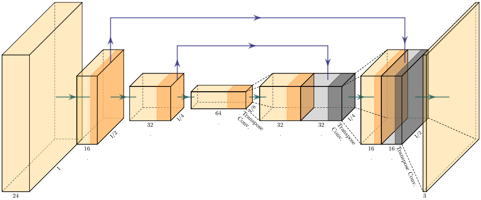
Fig. 4. Diagram of the network used to filter the hair. Convolutions are followed by a ReLU. Encoding steps are downsampling convolutions, while decoding steps are transpose convolutions set up to obtain outputs double the size of the input. All convolutions are followed by ReLU.
